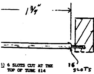
FIGURE FOUR SIDE VIEW OF COPPER TUBE, PAPER COILS AND ACRYLIC BASE
