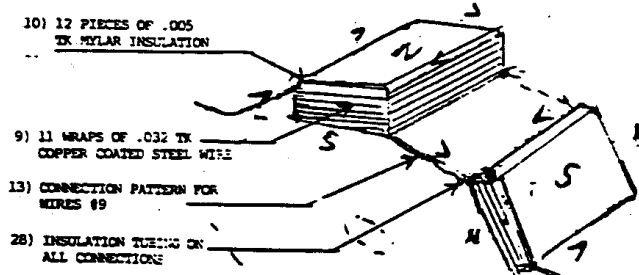
FIGURE SIX WIRE FLOW PATTERN (SOUTH HALF TO NORTH HALF)
