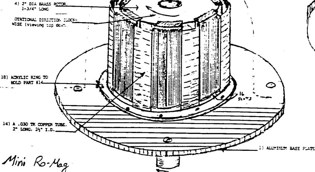
FIGURE TWO FULL SIZE ISOMETRIC 3) 5" DIA 4"
